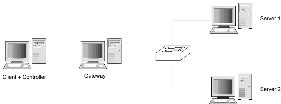
Abbildung 1: Experimental Setup
