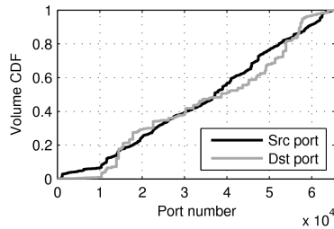
Fig. 4. Cumulative volume by the port number in k-2011
