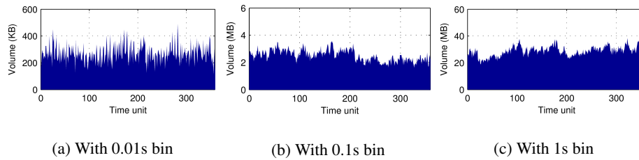
Fig. 7. Burstiness in aggregate UDP traffic from k-2011
